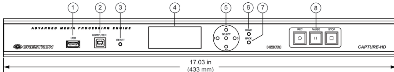
Capture Recorder Overall Dimensions – Front View (CAPTURE-HD Shown)
