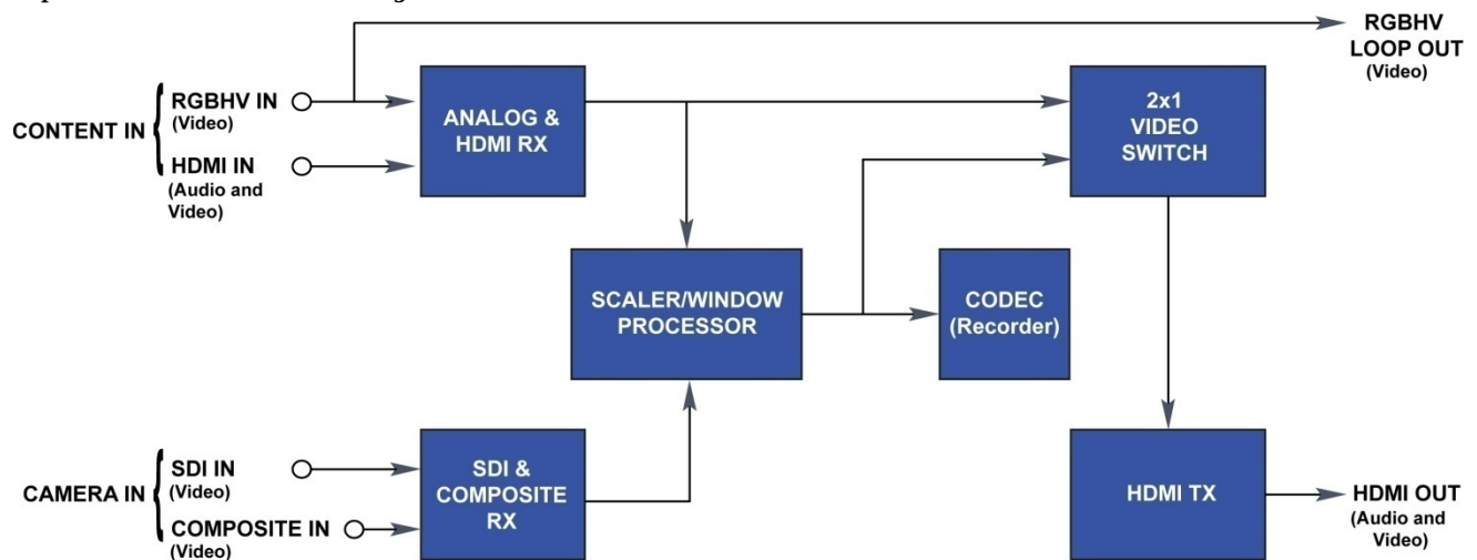
Capture Recorder Video Block Diagram
